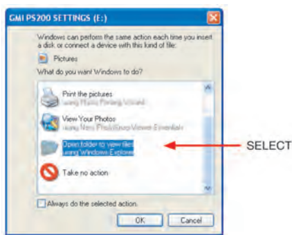
Fig. 3-1 Windows XP™
