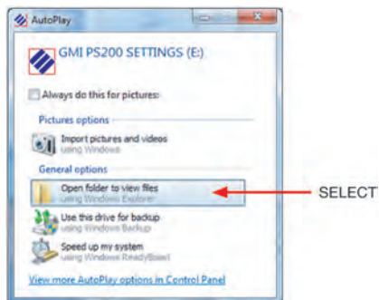
Fig. 3-3 Windows 7™
