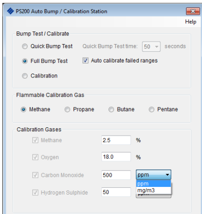
Fig. 3-11 Measurement Units
