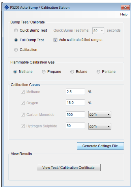
Fig. 3-16 Configuration Window
