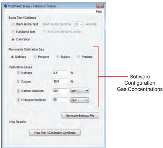
Fig. 2-3 Software Configuration
