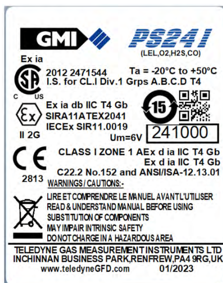
Figure 1-1: Identification Label
