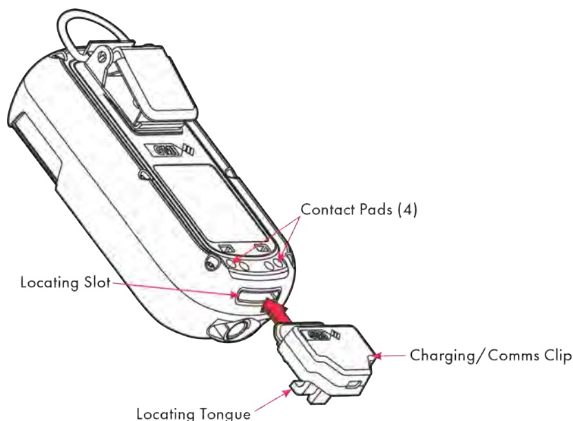
Figure 7-1: Charging/Comms Clip Connection
