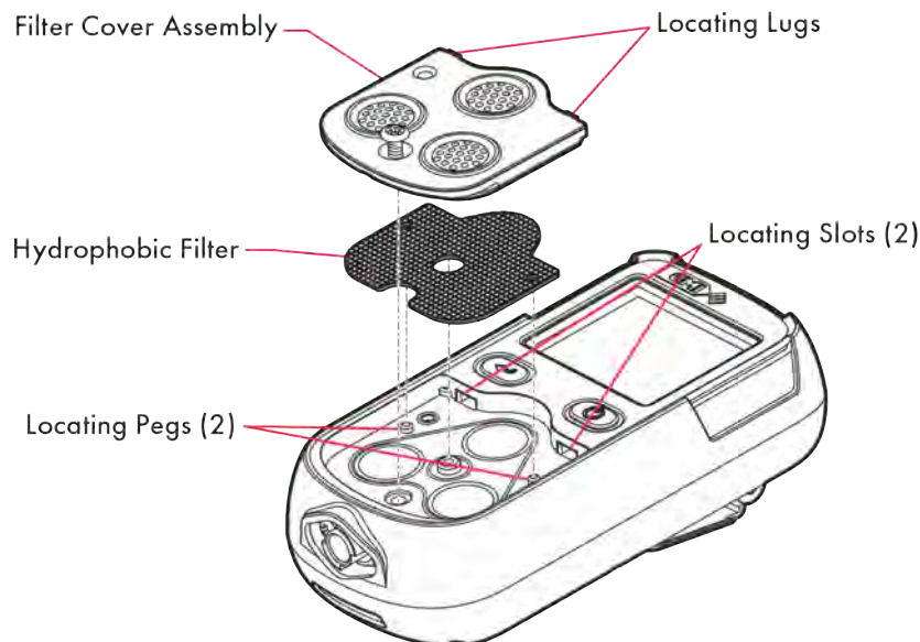
Figure 8-1: Hydrophobic Filter Replacement
