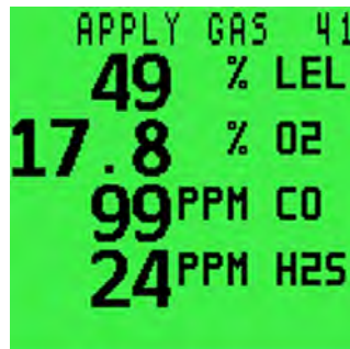
Figure 9-4: APPLY GAS Screen
