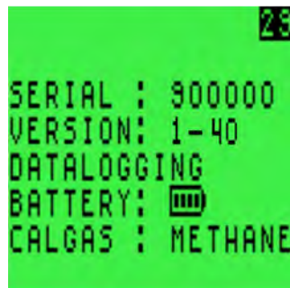
Figure 3-4: Monitor Identification Display
