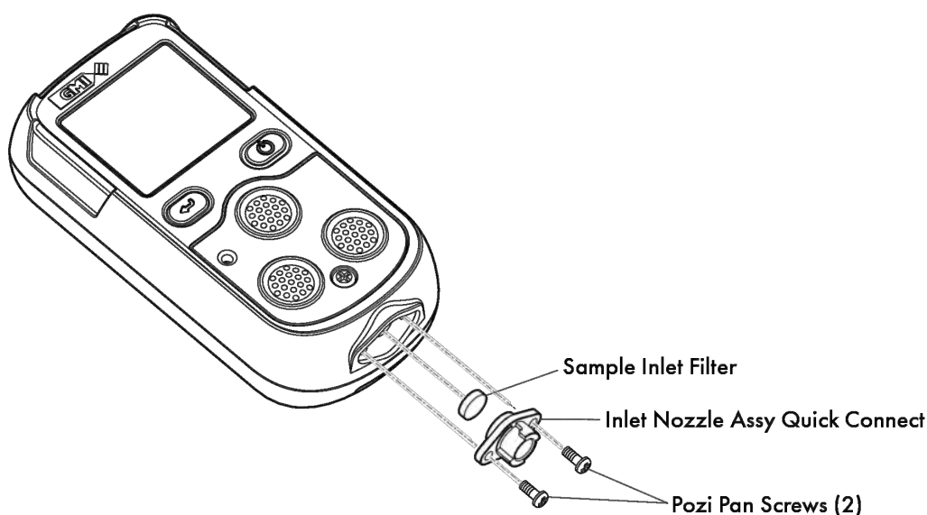
Figure 8-2: Replacing the Sample Inlet (Dust) Filter
