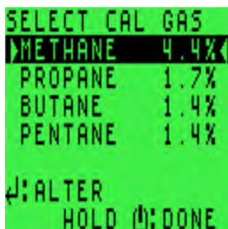
Figure 3-11: Cal Gas Selection
