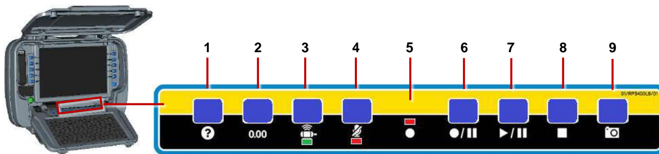
Fig. 3.6. Panel buttons
